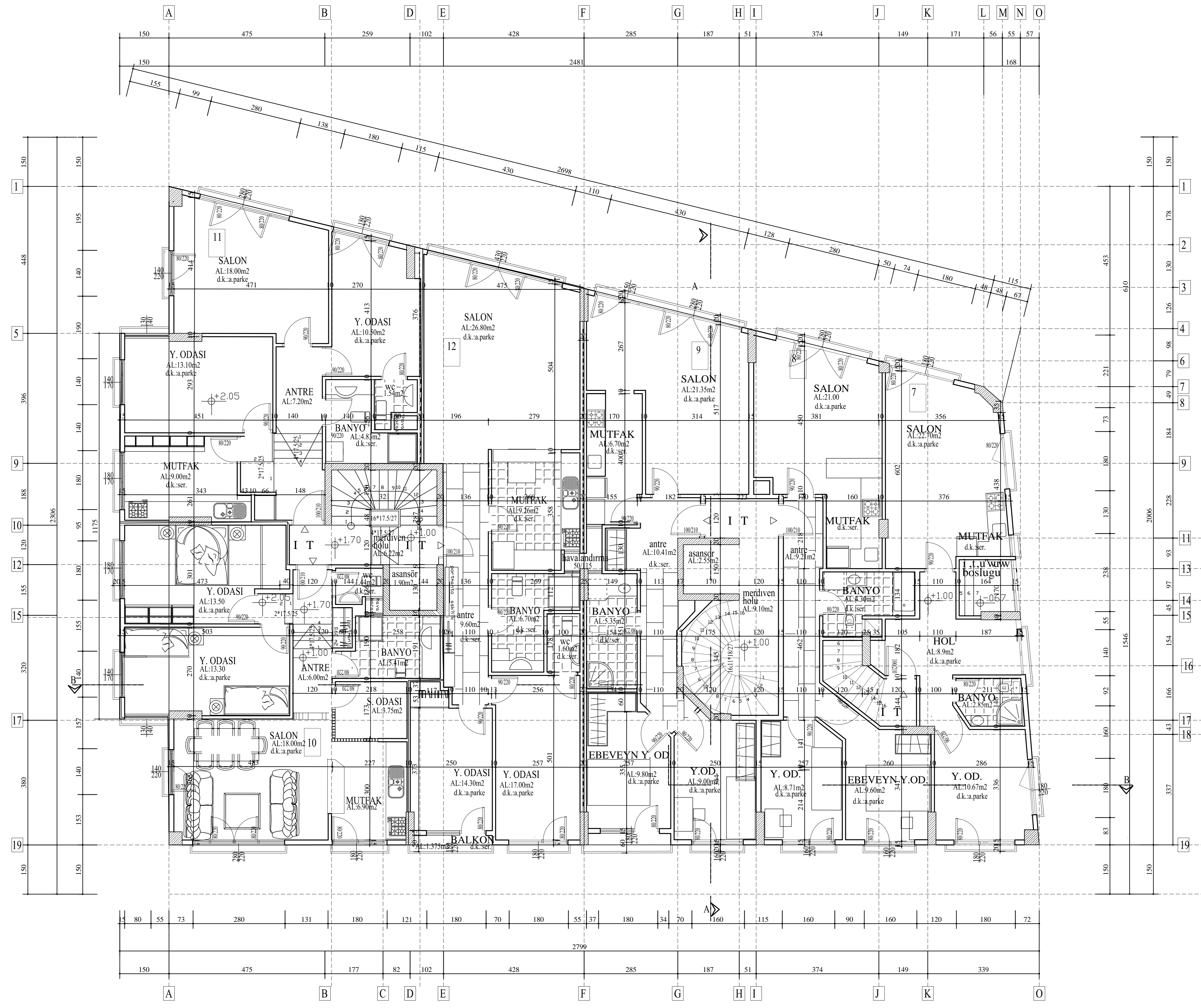
ZEMİN KAT PLANI Ö=1/50
